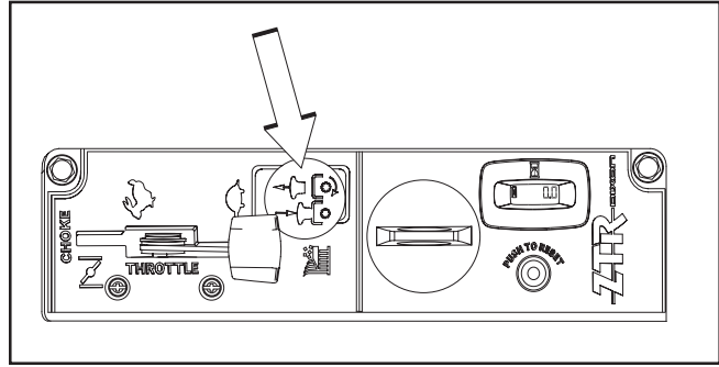
Blade switch
